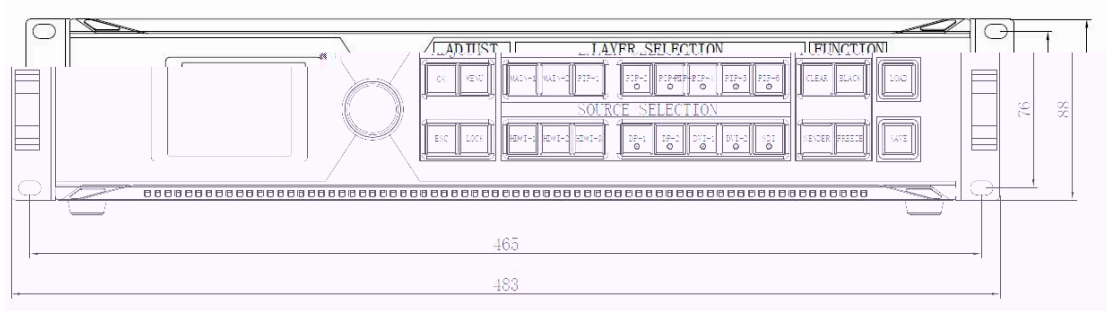
Front panel dimension drawing
