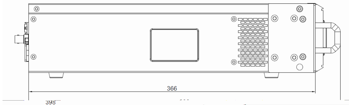
Side panel dimension drawing
